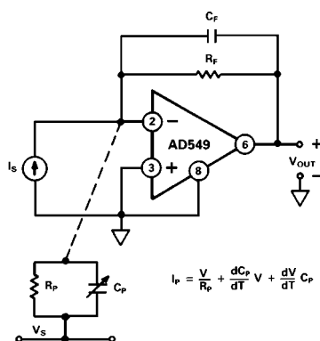
Figure 26. Sources of Parasitic Leakage Currents
