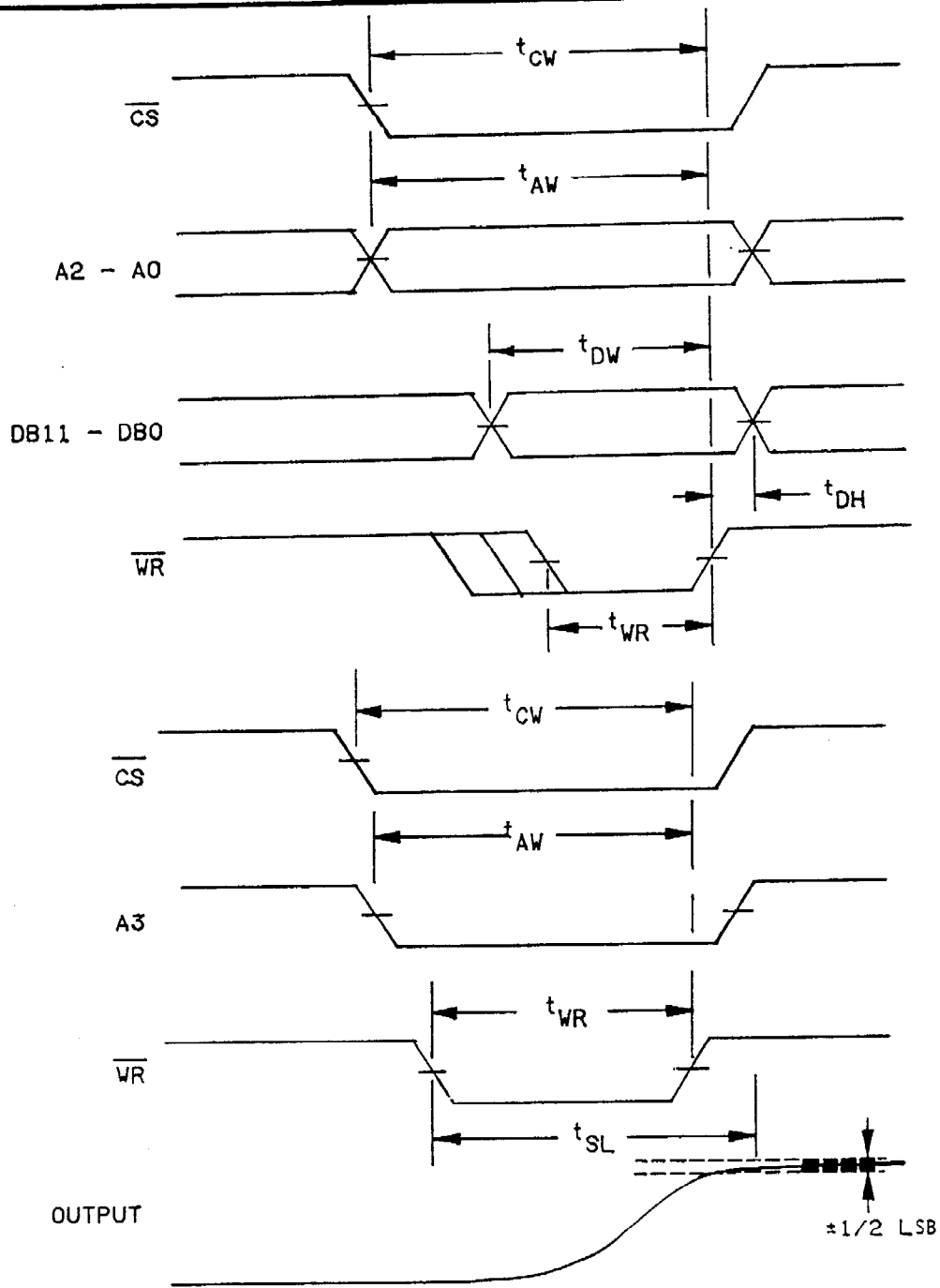
FIGURE 4. Switching waveforms.
