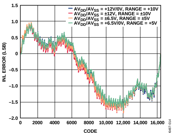
Figure 7. AD5732 Integral Nonlinearity Error vs. Code
