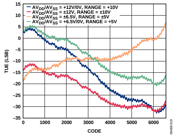
Figure 35. AD5754 Total Unadjusted Error vs. Code
