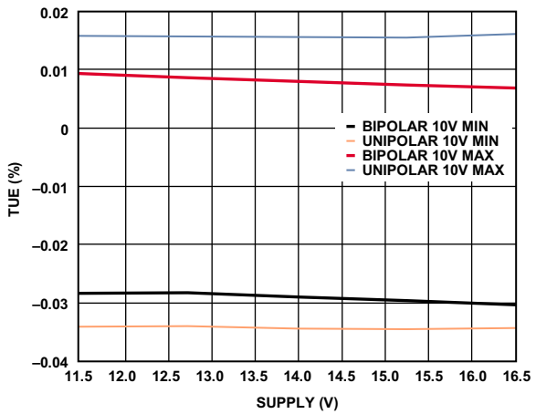
Figure 18. AD5754R Total Unadjusted Error vs. Supply Voltage
