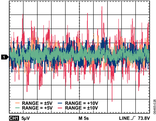
Figure 30. Peak-to-Peak Noise, 0.1 Hz to 10 Hz Bandwidth
