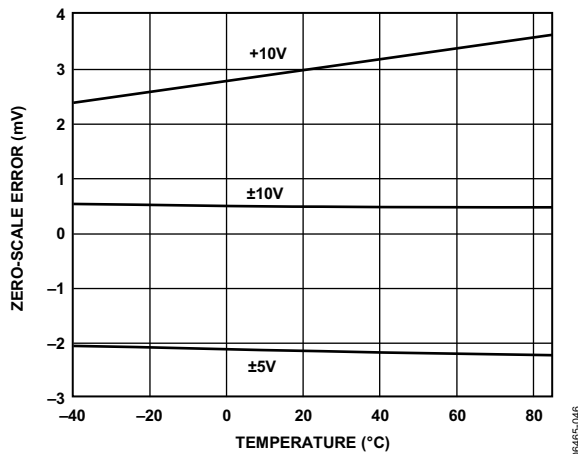
Figure 20. Zero-Scale Error vs. Temperature
