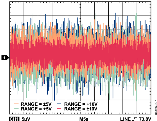
Figure 31. Peak-to-Peak Noise, 100 kHz Bandwidth
