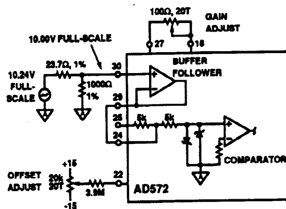
Figure 10. Analog Input Connections for Unipolar 0 to +10.24 V Input Range
