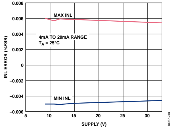
Figure 17. Integral Nonlinearity Error vs. Supply, External R_{SET}
