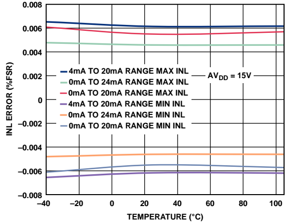
Figure 12. Integral Nonlinearity Error vs. Temperature, External R_{SET}
