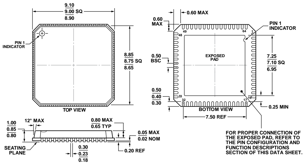
COMPLIANT TO JEDEC STANDARDS MO-220-VMM4 Figure 66. 64-Lead Lead Frame Chip Scale Package [LFCSP_VQ] 9 mm × 9 mm Body, Very Thin Quad (CP-64-3) Dimensions shown in millimeters
