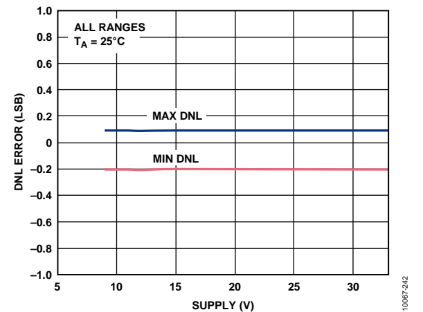
Figure 19. Differential Nonlinearity Error vs. Supply
