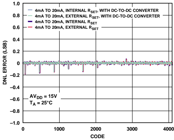
Figure 9. Differential Nonlinearity Error vs. DAC Code
