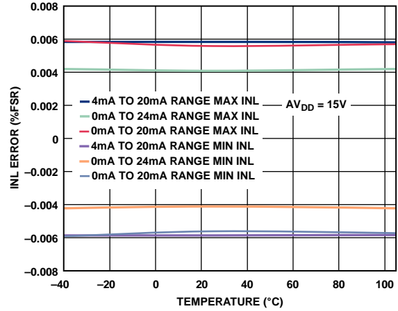
Figure 11. Integral Nonlinearity Error vs. Temperature, Internal R_{SET}
