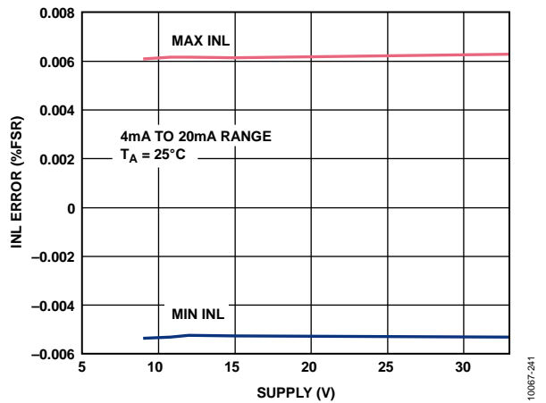
Figure 18. Integral Nonlinearity Error vs. Supply, Internal R_{SET}
