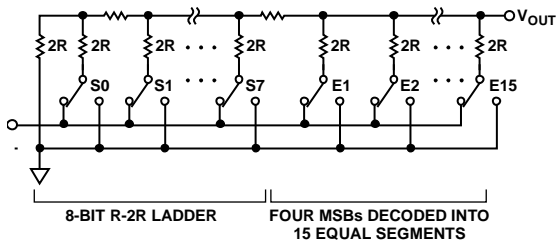
Figure 47. DAC Ladder Structure
