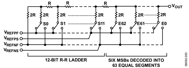
Figure 49. DAC Ladder Structure Serial Interface
