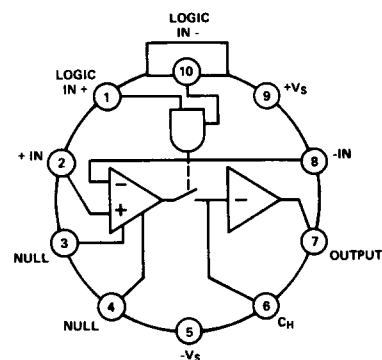
10 PIN TO-100
