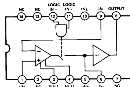
14 PIN DIP
