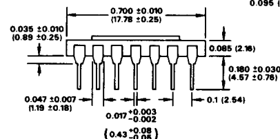
TO-116 "D"
