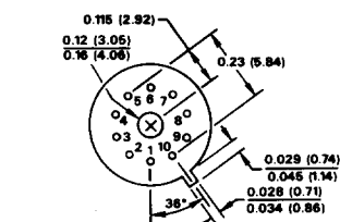
TO-100 "H"
