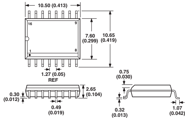
Dimensions shown in millimeters and (inches) 16-Lead SOIC Package (R-16)
