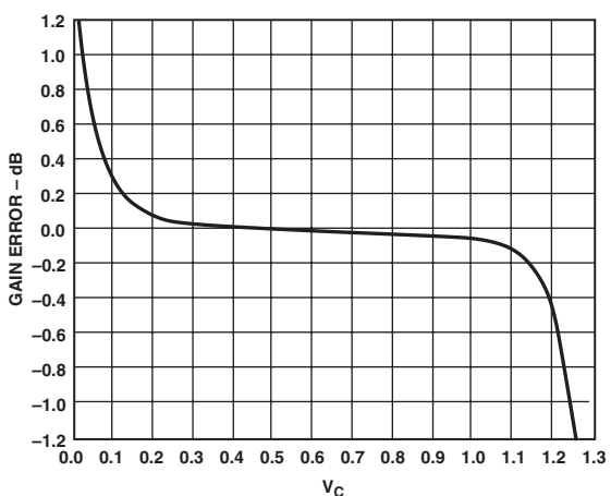
Figure 9. Gain Error for Cascaded Stages — Low Ripple Mode
