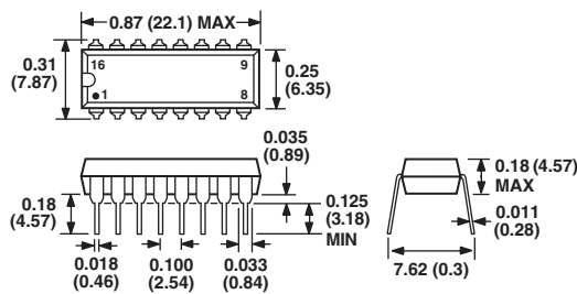
Dimensions shown in inches and (mm) 16-Lead Plastic DIP Package (N-16)
