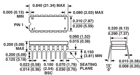
Dimensions shown in inches and (mm) 16-Lead Cerdip Package (Q-16)
