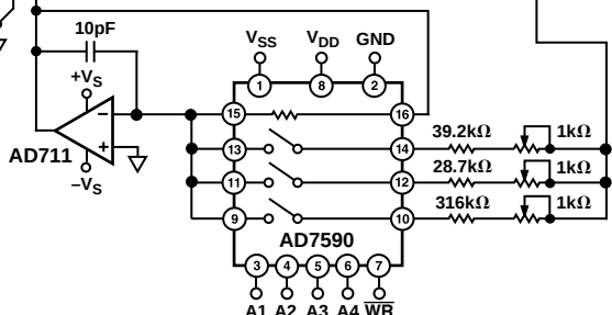
Figure 39. Programmable Output Gain
