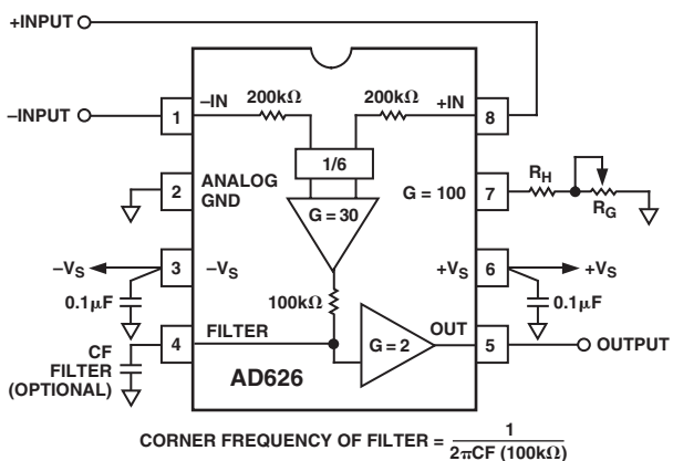
RESISTOR VALUES FOR GAIN ADJUSTMENT
