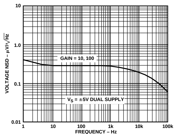
Figure 15. Noise Voltage Spectral Density vs. Frequency
