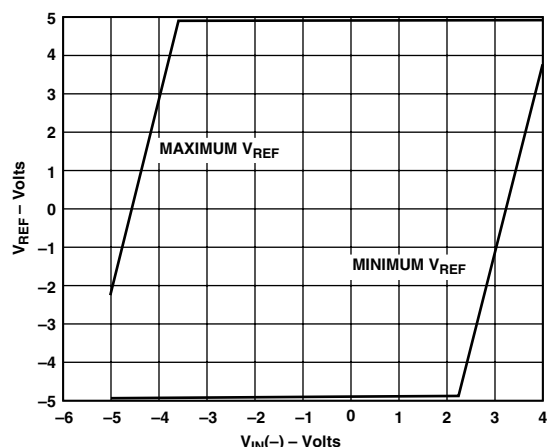
Figure 5. Reference Input Voltage vs. Negative Input Voltage, V_S = \pm 5 V, G = +5
