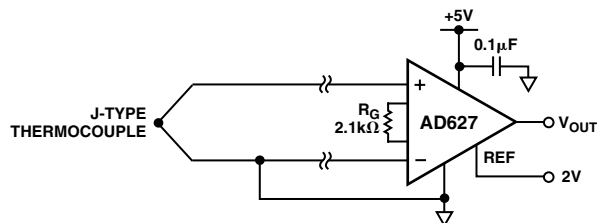
Figure 17. Amplifying Bipolar Signals with Low Common-Mode Voltage
