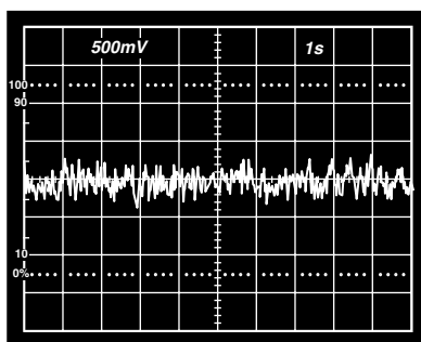
TPC 7. 0.1 Hz to 10 Hz Current Noise (0.71 pA/DIV)
