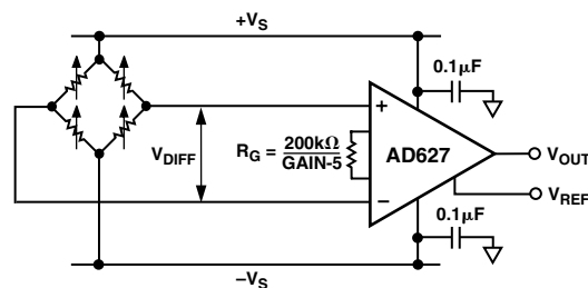
Figure 15. A Classic Bridge Circuit
