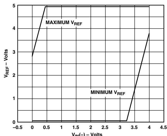
Figure 6. Reference Input Voltage vs. Negative Input Voltage, V_S = 5 V, G = +5
