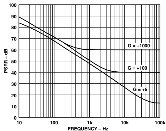
TPC 11. Negative PSRR vs. Frequency, \pm 5V
