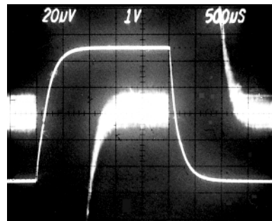
TPC 18. Large Signal Pulse Response and Settling Time, G = -1000 , R_L = 20 \text{ k}\Omega , C_L = 100 \text{ pF} ( 10 \mu\text{V} = 0.01\% )
