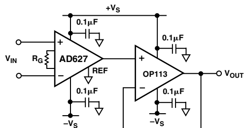
Figure 7. Output Buffering
