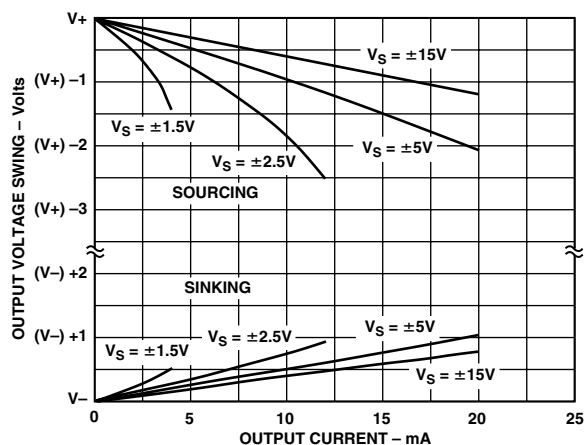
TPC 6. Output Voltage Swing vs. Output Current
