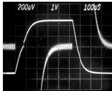
TPC 17. Large Signal Pulse Response and Settling Time, G = -100 , R_L = 20 \text{ k}\Omega , C_L = 100 \text{ pF} ( 100 \mu\text{V} = 0.01\% )
