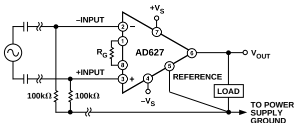
Figure 41c. Ground Returns for Bias Currents with AC Coupled Inputs
