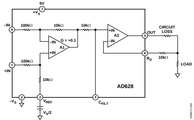
Figure 35. Kelvin Connection
