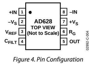
Figure 4. Pin Configuration
