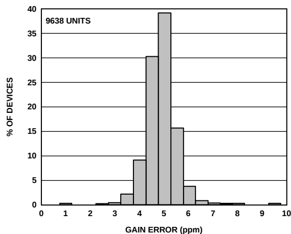
Figure 14. Typical Distribution of +1 Gain Error
