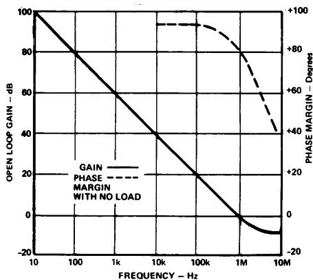
Figure 10. Open Loop Frequency Response
