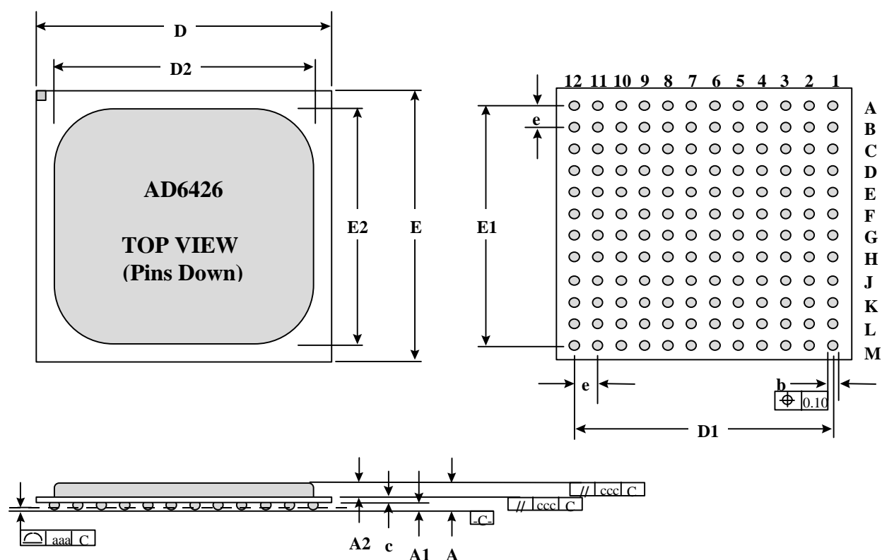
PBGA Outline Dimensions
