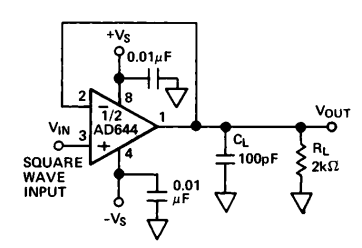
Figure 21c. Unity Gain Follower
