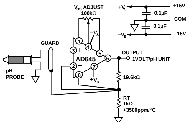
Figure 35. A pH Probe Amplifier
