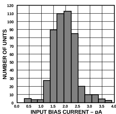
Figure 5. Typical Distribution of Input Bias Current (576 Units)
