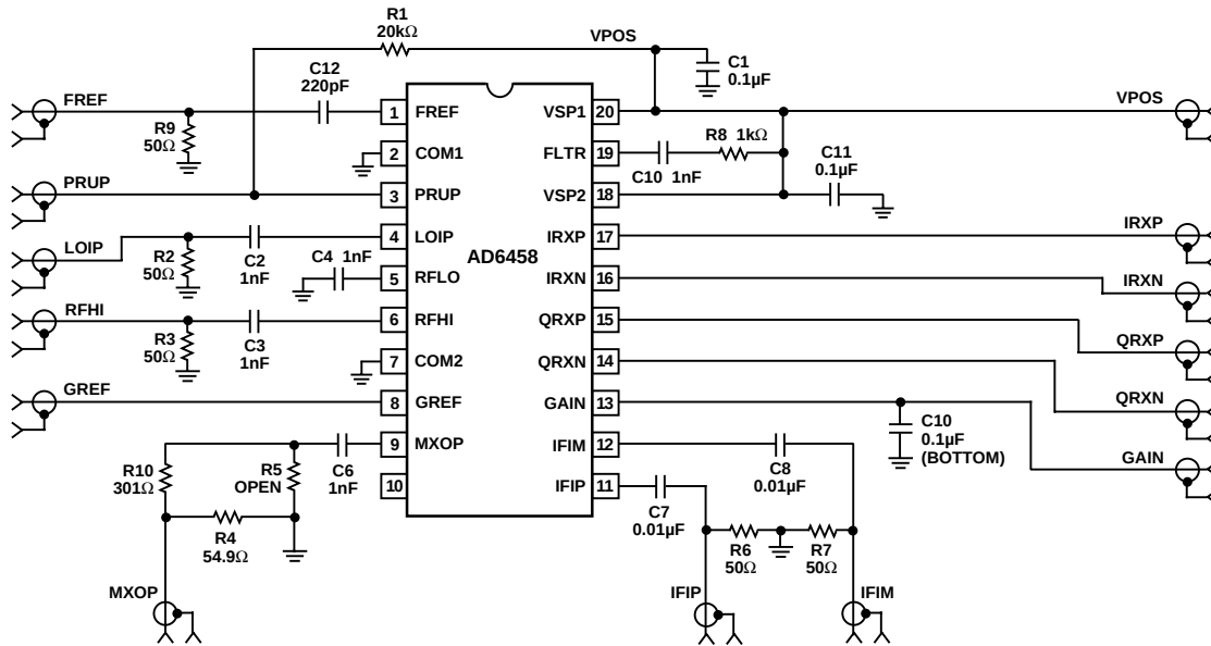
Figure1. Characterization Board
