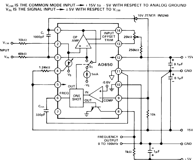
Figure 12. Differential Input
