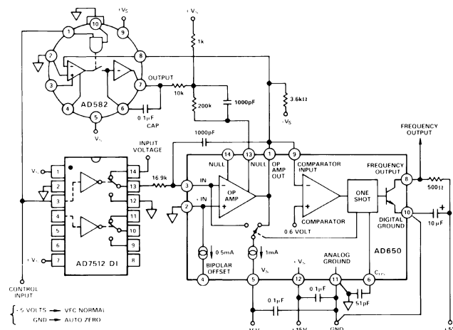
Figure 13. Autozero Circuit
