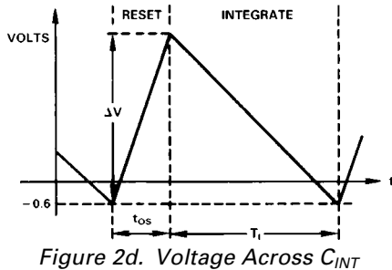
Figure 2d. Voltage Across C_{INT}
