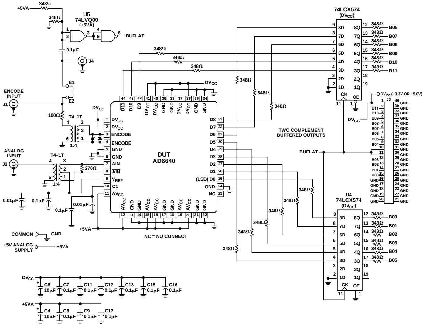
Figure 36. AD6640ST/PCB Schematic
