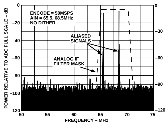
Figure 21. IF-Sampling at 70 MHz without Dither
