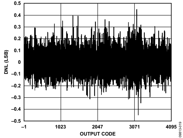
Figure 19. DNL; 500 MSPS
