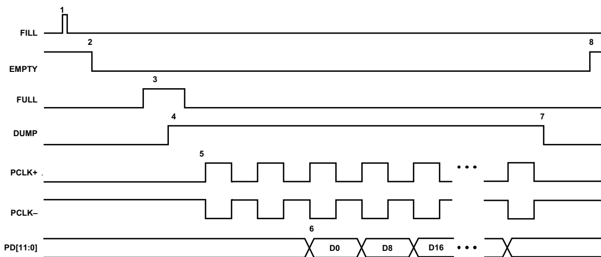
Figure 40. Parallel Mode Transaction Diagram
