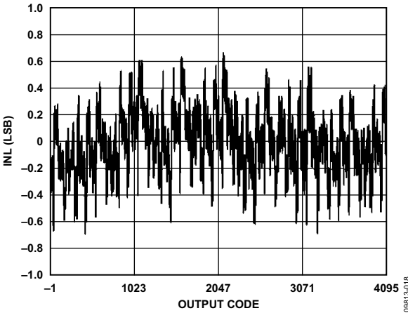
Figure 18. INL; 500 MSPS
