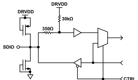
Figure 33. Equivalent SDIO Circuit
