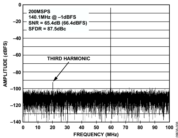
Figure 8. AD6643-200 Single Tone FFT, f_{IN} = 140.1 MHz
