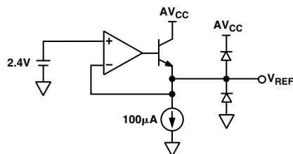
Figure 6. 2.4 V Reference
