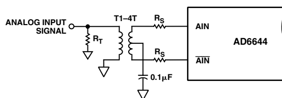
Figure 27. Transformer-Coupled Analog Input Circuit
