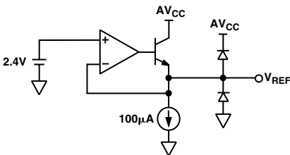
Figure 6. 2.4 V Reference
