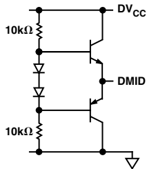
Figure 7. DMID Reference
