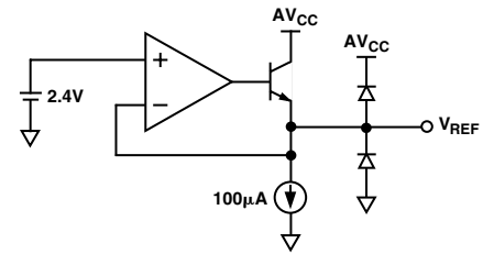
Figure 6. 2.4 V Reference
