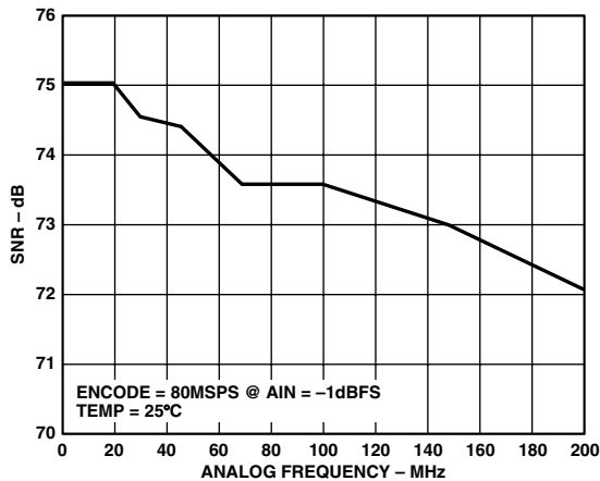
TPC 9. Noise vs. Analog Frequency (IF)
