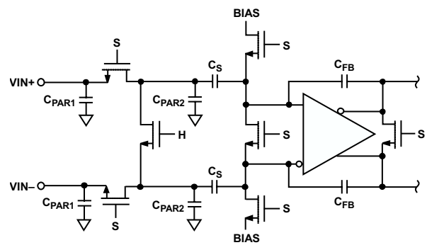
Figure 26. Switched-Capacitor Input
