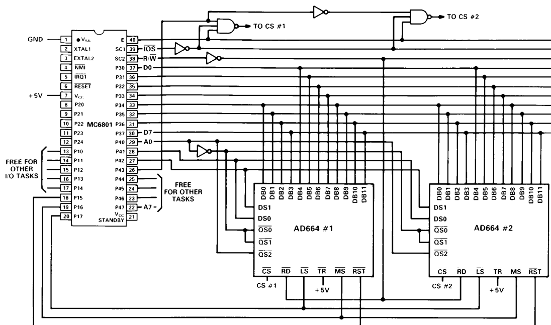
Figure 25c. Interfacing Two AD664s to an MC6801
