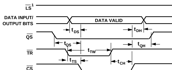
Figure 18a. Fully Transparent Mode
