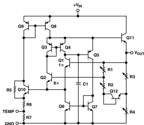
Figure 2. Schematic Diagram
