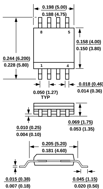
8-Pin SOIC
