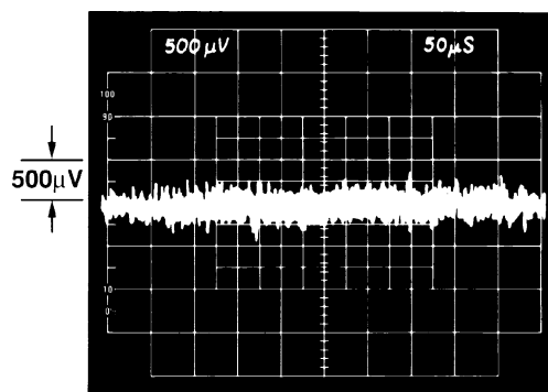
Figure 4. Broadband Noise at 300 kHz
