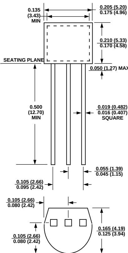
3-Pin TO-92
