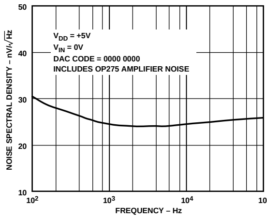
Figure 13. Noise Spectral Density vs. Frequency
