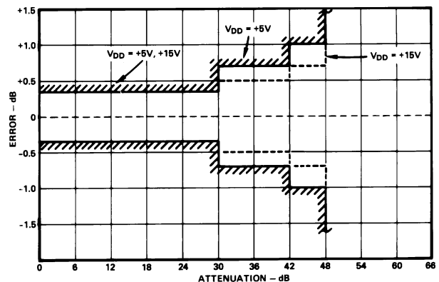
Accuracy Specification for L/C/U Grade Devices at T_A = +25^\circ\text{C} REV. A
