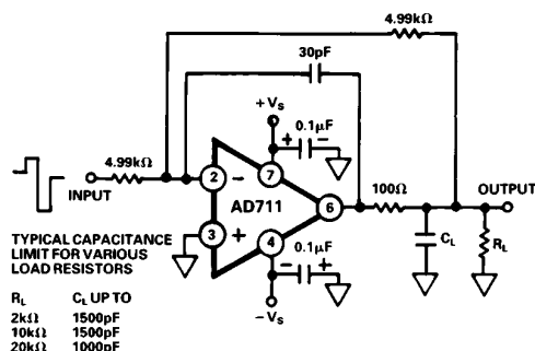
Figure 36. Circuit for Driving a Large Capacitive Load
