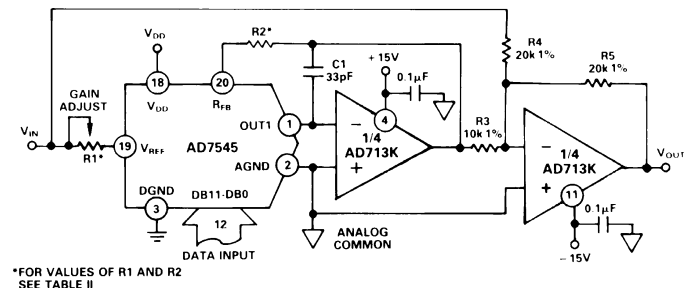
Figure 17. Bipolar Operation
