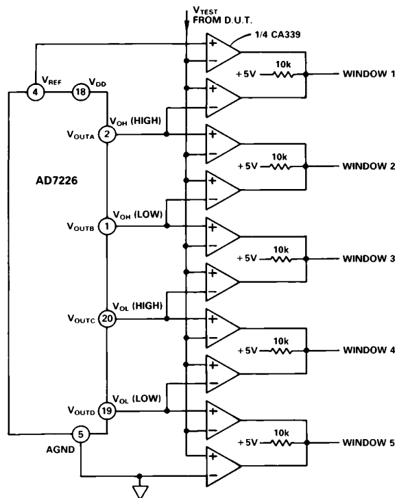
Figure 18a. Logic Level Measurement
