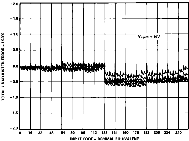
Figure 6. Channel-to-Channel Matching
