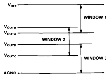
Figure 19b. Window Structure
