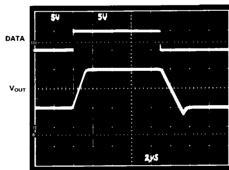
Figure 10. Dynamic Response ( V_{SS} = -5\text{ V} )
