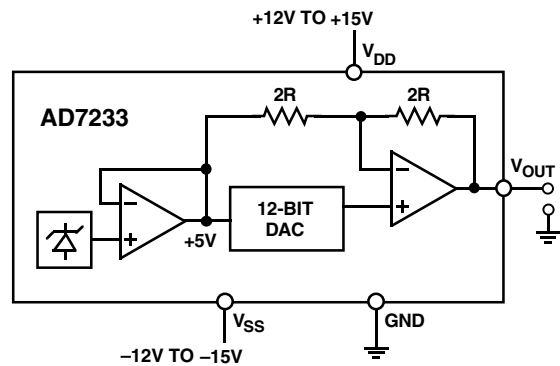
Figure 4. Circuit Configuration
