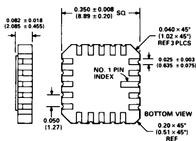
20-Terminal Leadless Ceramic Chip Carrier (E-20A)
