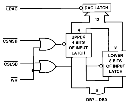
Figure 6. AD7248A Input Control Logic
