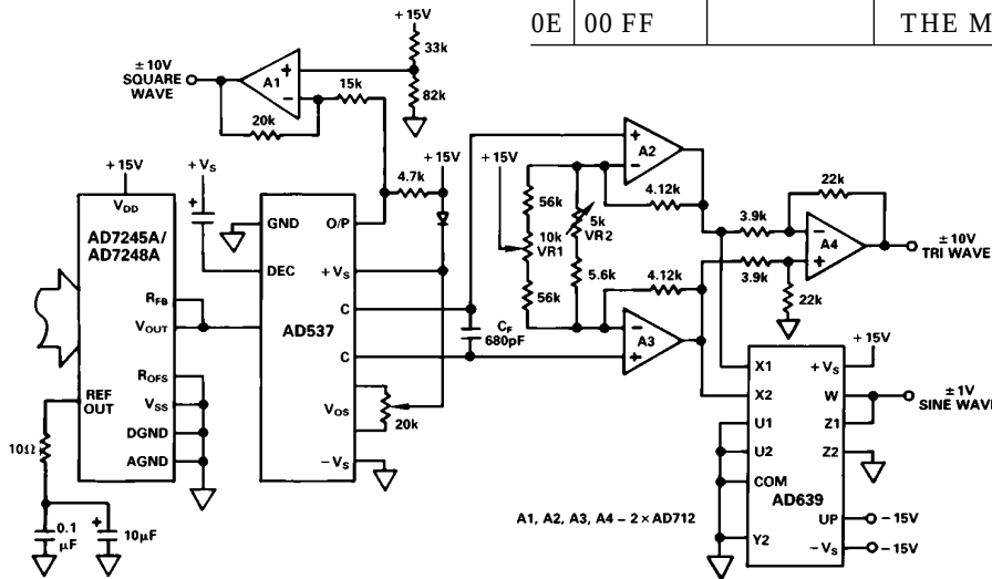
Figure 11. Programmable Function Generator
