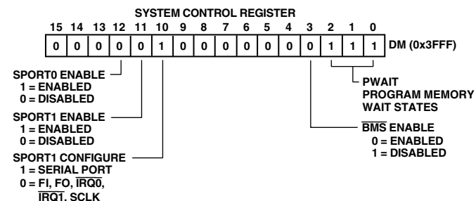
Figure 17. System Control Register
