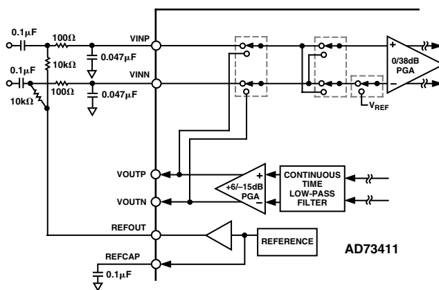
Figure 27. Analog Input (AC-Coupled) Differential
