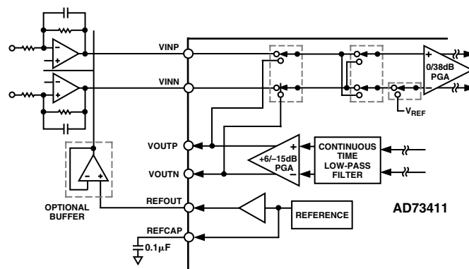
Figure 26. Analog Input (DC-Coupled) Using External Amplifiers
