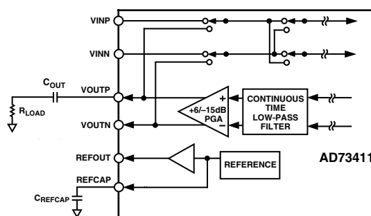
Figure 32. Example Circuit for Single-Ended Output
