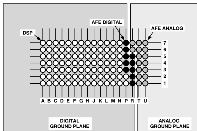
Figure 34. Ground Plane Layout
