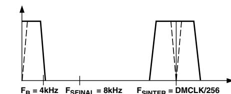
d. Final Filter LPF (HPF) Transfer Function
