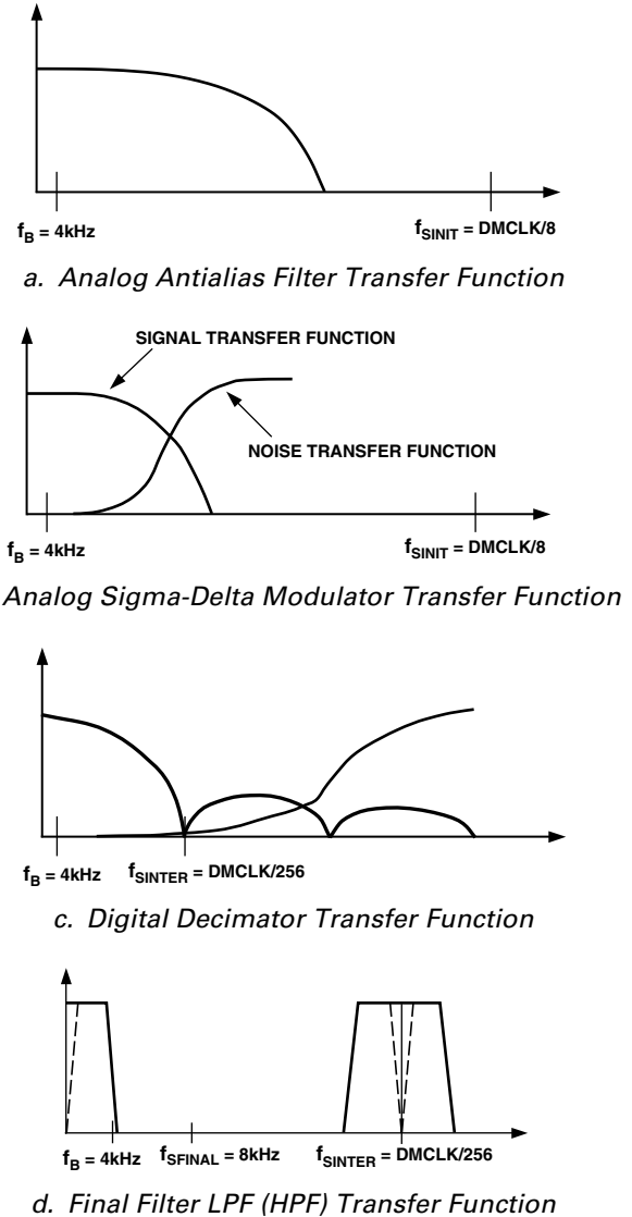
Figure 4. DC Frequency Responses
