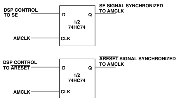
Figure 21. SE and ARESET Sync Circuit for Cascaded Operation
