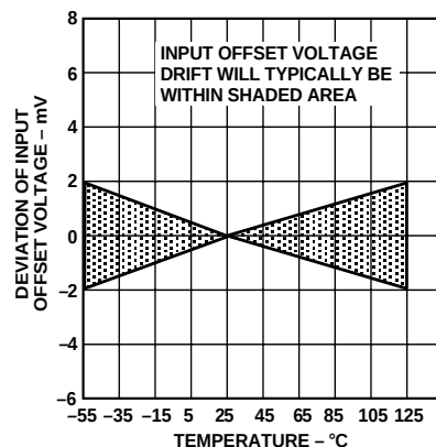
Figure 36. V_{OS} Drift, Y Input
