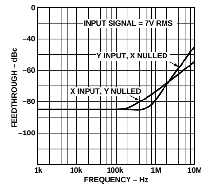
Figure 25. Feedthrough vs. Frequency
