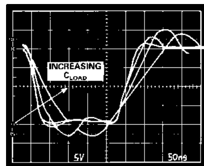
Figure 31. Pulse Response vs. C_{LOAD} , C_{LOAD} = 0 pF, 47 pF, 100 pF, 200 pF
