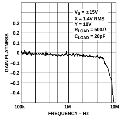
Figure 22. Gain Flatness, 300 kHz to 10 MHz, R_L = 500\text{ }\Omega
