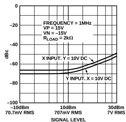
Figure 28. THD vs. Signal Level, f = 1\text{ MHz}
