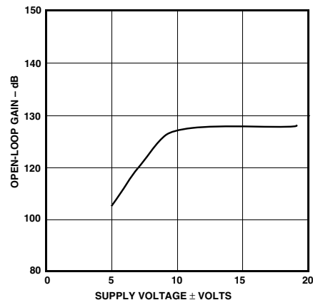
TPC 12. Open-Loop Gain vs. Supply Voltage, R_{LOAD} = 2K
