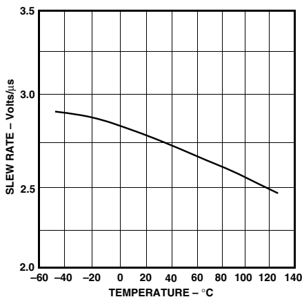
TPC 11. Slew Rate vs. Temperature (Gain = -1)
