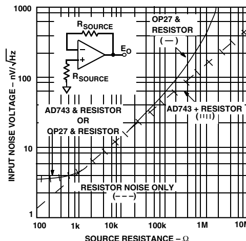
Input Noise Voltage vs. Source Resistance
