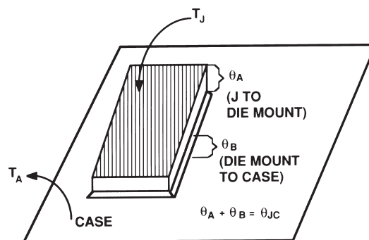
Figure 10. A Breakdown of Various Package Thermal Resistances
