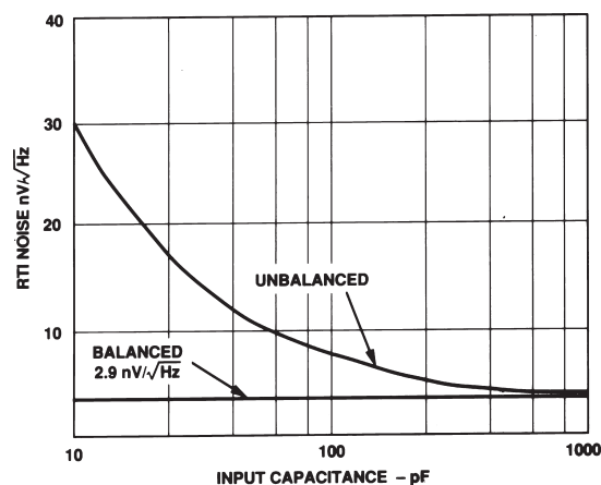
Figure 15. RTI Voltage Noise vs. Input Capacitance
