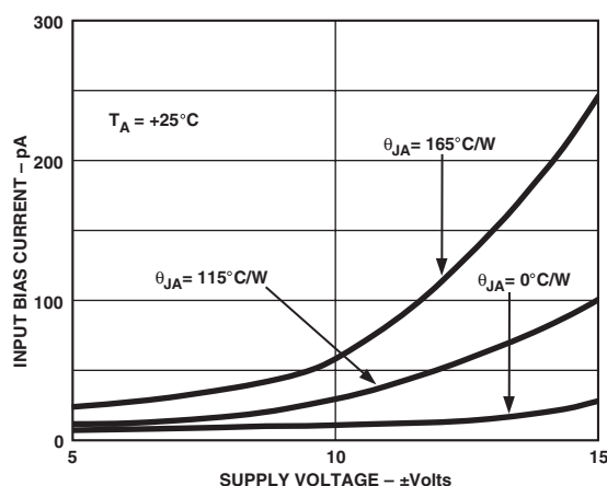
Figure 9. Input Bias Current vs. Supply Voltage for Various Values of \theta_{JA}
