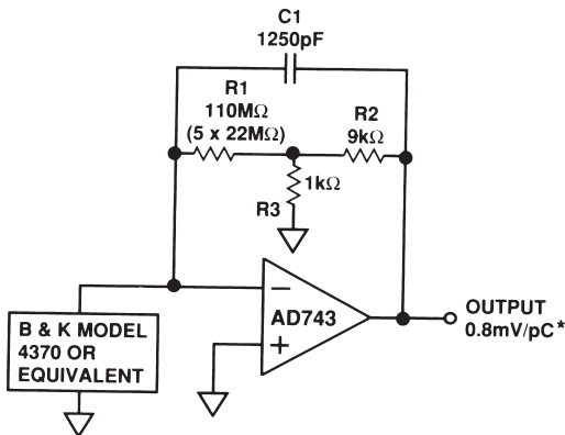
Figure 13a. A Basic Accelerometer Circuit
