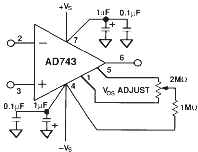
TPC 20. Offset Null Configuration
