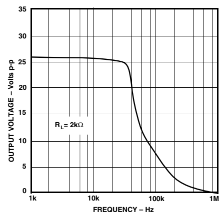
TPC 15. Large Signal Frequency Response
