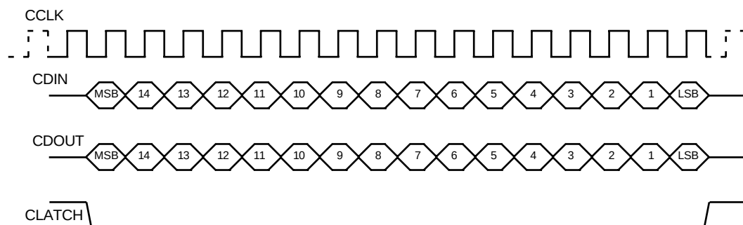
Figure &lt;Control_Timing&gt;
