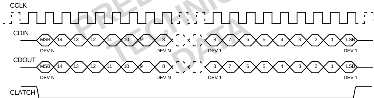
Figure &lt;Control_Cascade_Timing_Daisy_Chain&gt;
