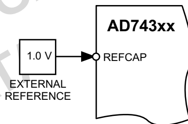
Figure &lt;REFCAP_Ext&gt;
