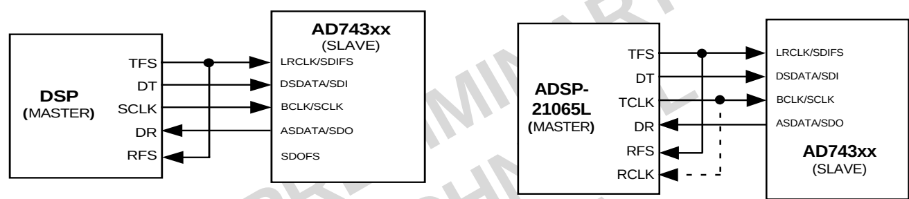
Figure <Data_DSP_Master>
