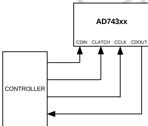
Figure &lt;Control_Interface&gt;
