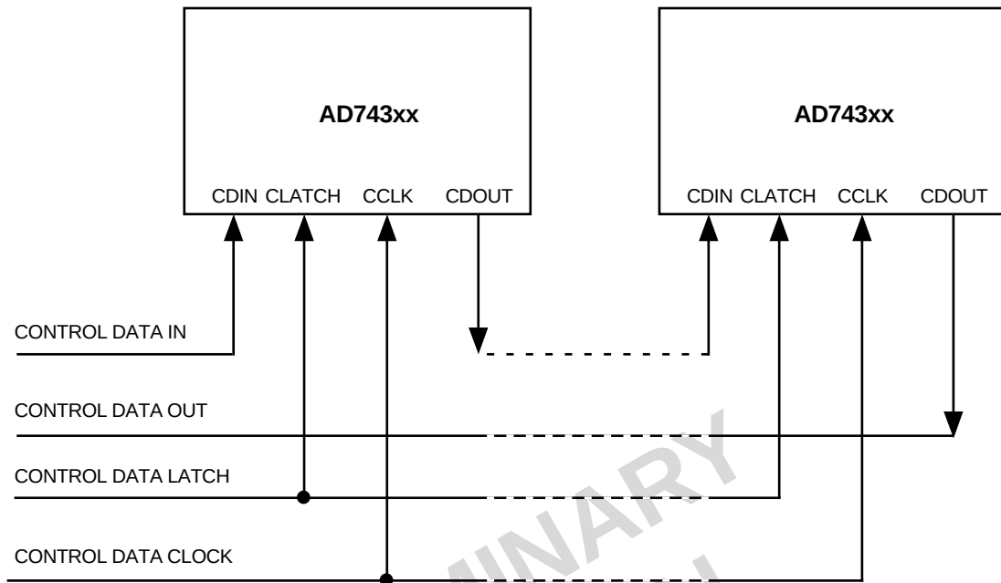
Figure &lt;Control_Cascade_Daisy_Chain&gt;
