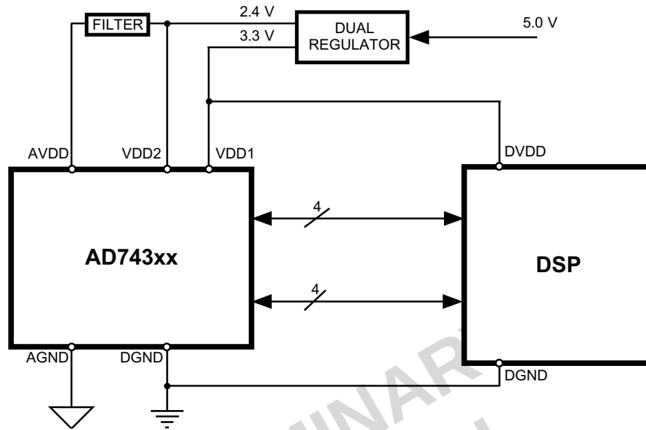
Figure &lt;PSU_Connection&gt;
