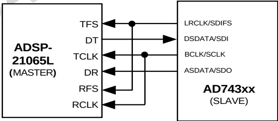
Figure <Data_I2S_DSP_Slave>
