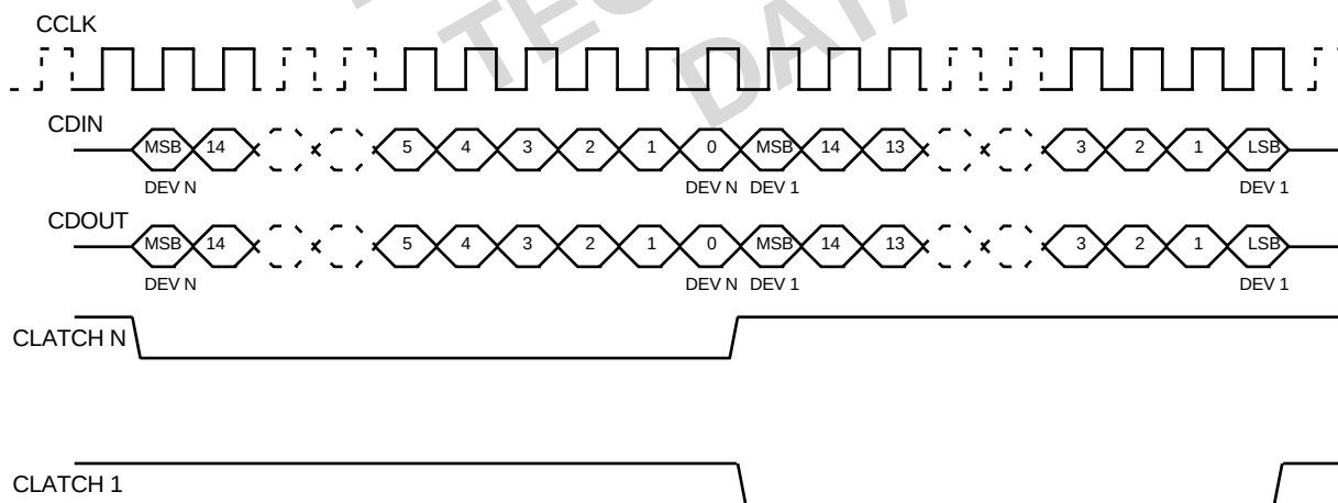
Figure <Control_Cascade_Timing_TDM>
