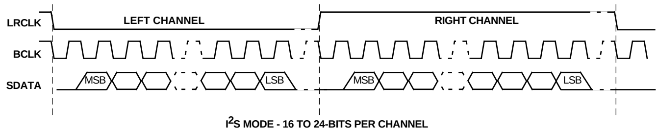
Figure <I2S_Timing>
