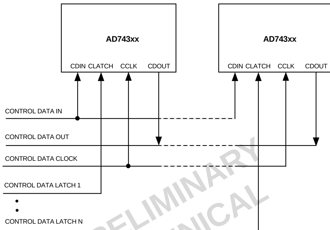
Figure <Control_Cascade_TDM>
