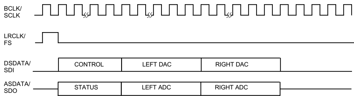
Figure <DSP_Protocol>
