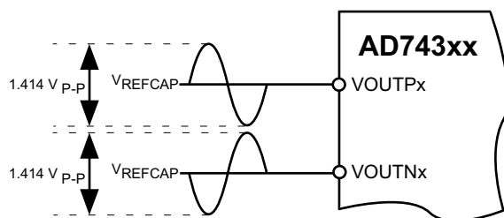
Figure &lt;Output_Swing&gt;
