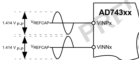
Figure &lt;Input_Swing&gt;
