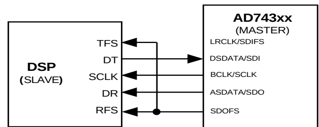
Figure &lt;Data_DSP_Slave&gt;
