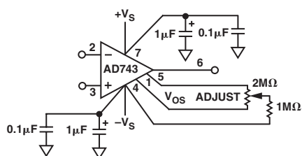
TPC 20. Offset Null Configuration
