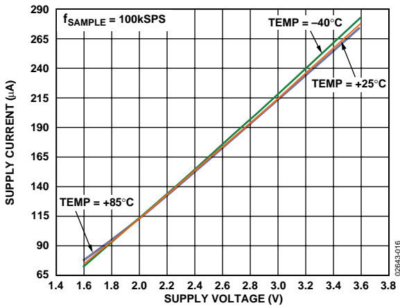
Figure 16. Supply Current vs. Supply Voltage, SCLK 3.4 MHz
