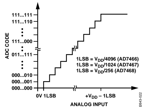
Figure 22. AD7466/AD7467/AD7468 Transfer Characteristics
