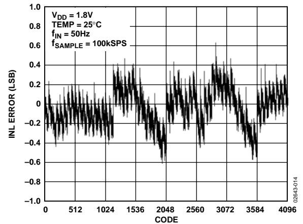
Figure 14. AD7466 INL Performance
