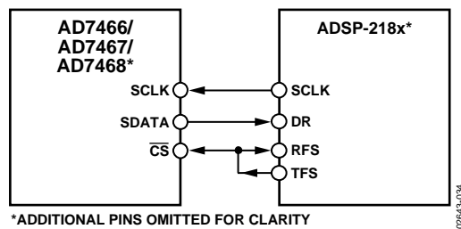
Figure 34. Interfacing to the ADSP-218x
