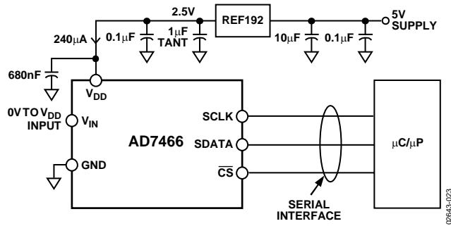
Figure 23. REF192 as Power Supply to AD7466
