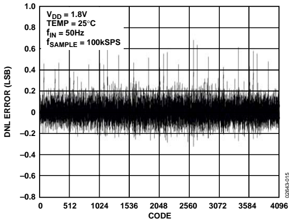
Figure 15. AD7466 DNL Performance
