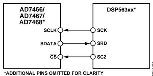
Figure 35. Interfacing to the DSP563xx
