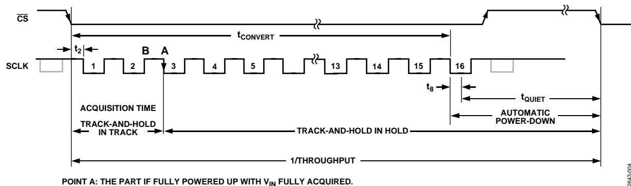
Figure 4. AD7466 Serial Interface Timing Diagram Example
